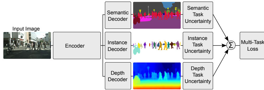
Figure 4.2: Visual example of a Multi-task deep learning model. Homoscedastic Task Uncertainty is introduced as a principled way of combining multiple regression and classification loss functions for multi-task learning. As an example, the architecture takes a single monocular RGB image as input and produces a pixel-wise classification, an instance semantic segmentation and an estimate of per pixel depth. Notice that Multi-task learning can improve accuracy over separately trained models because cues from one task, such as depth, are used to regularize and improve the generalization of another domain, such as segmentation. From [KGC18].
