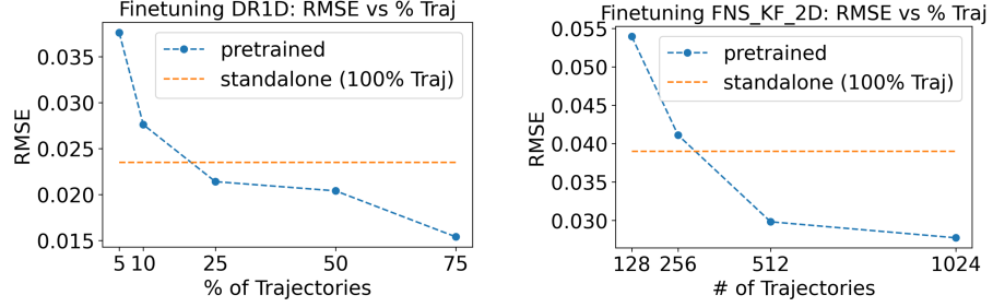
(a) 1D Diffusion–Reaction task.
