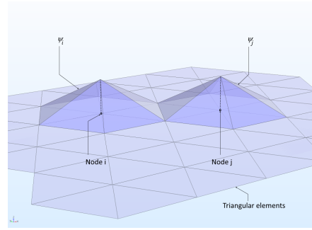
(b) No overlap between basis functions. From [Mul].
