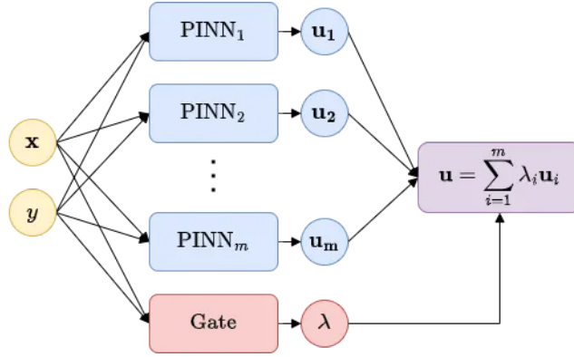
Figure 4.15: Mixture of Experts of PINNs. An arbitrary number m of PINNs, possibly with varying architectures and properties, is initialised together with a gating network. All models receive the same input and the gate produces weights that are used for aggregating the results. From [BK22].
