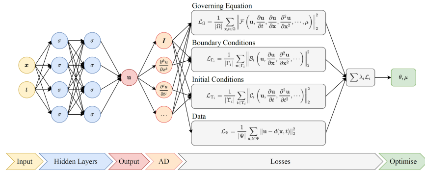
Figure 3.1: Visual representation of a PINN. From here.
