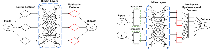
(a) Multi-scale Fourier feature architecture : multiple Fourier feature embeddings (initialised with different \sigma ) are applied to input coordinates and then passed through the same fully-connected neural network, before the outputs are finally concatenated with a linear layer. From [WWP21b].
