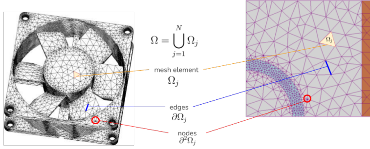
Figure 2.6: Visual representation of the meshing of the domain \Omega for the FEM analysis (2D surface in 3D space on the left, and a plain 2D region on the right). Adapted from [BCT02].
