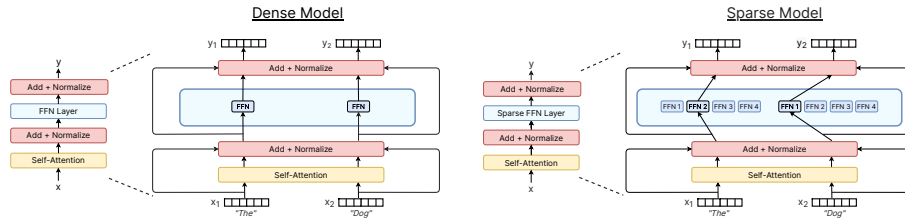
Figure 4.14: Comparing a dense and sparse expert Transformer. A dense model ( left ) sends both input tokens to the same feed-forward network parameters (FFN). A sparse expert model ( right ) routes each input token independently among its four experts (FFN1 \dots FFN4). In this diagram, each model uses a similar amount of computation, but the sparse model has more unique parameters. Note while this figure showcases a specific and common approach of sparse feed-forward network layers in a Transformer [Vas+17], the technique is more general. From [FDZ22]
