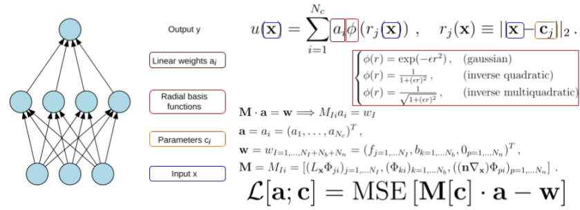
Figure 2.11: Visual representation of the Kansa method.
