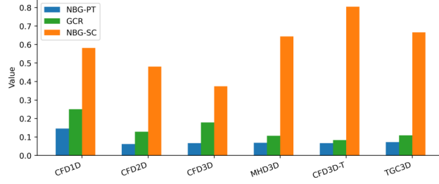
Figure 5.25: Zero-shot Gap-Closure Ratio (GCR) for MORPH pretrained on 2D incompressible Navier–Stokes and evaluated on six out-of-distribution targets. Positive GCR across all targets indicates successful transfer across modalities and physics. Adapted from [Rau+25].
