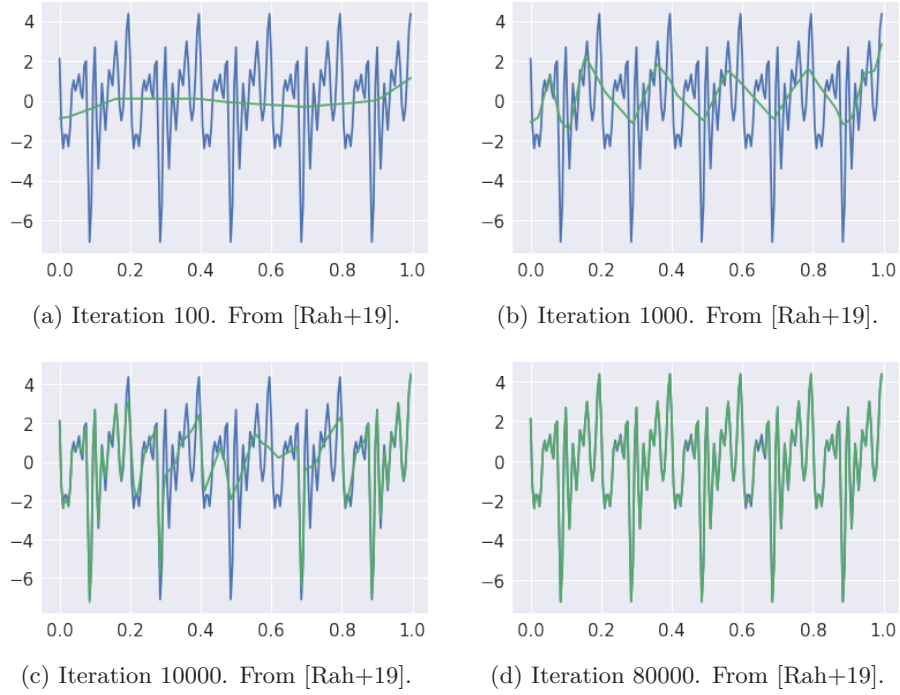
Figure 4.7: The learnt function (green) overlayed on the target function (blue) as the training progresses. The target function is a superposition of sinusoids of frequencies \kappa = (5, 10, \dots, 45, 50) , equal amplitudes and randomly sampled phases. From [Rah+19].
