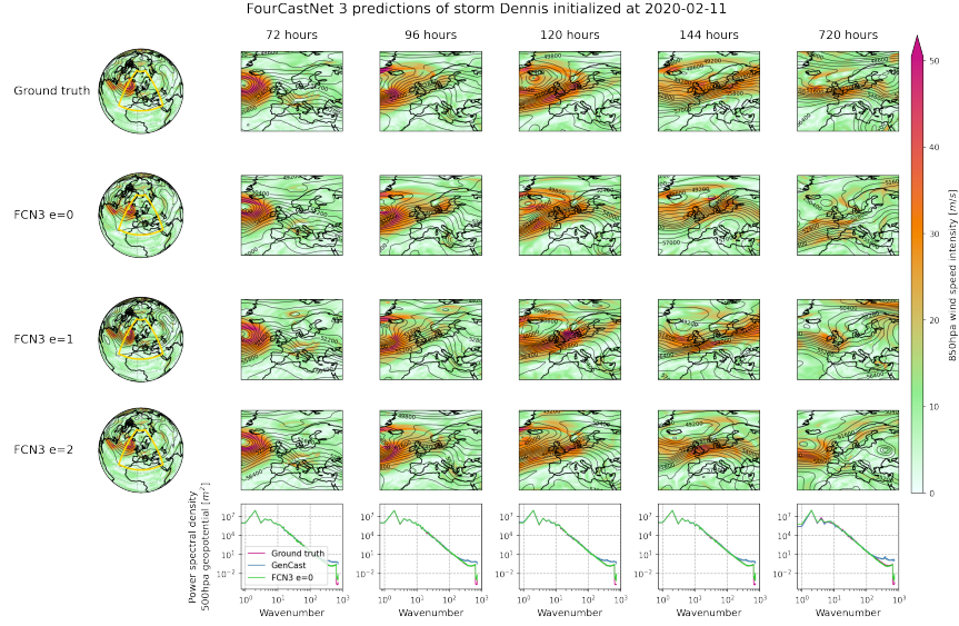
Figure 5.17: FourCastNet 3 prediction of storm Dennis initialized on 2020-02-11 at 00:00:00 UTC. The plot depicts wind-speeds at a pressure level of 850hPa and isohypses (height contours) of the 500hPa geopotential height. FCN3 accurately predicts the storm and its landfall 5 days in advance, with different ensemble members depicting different scenarios. FCN3 predicts global weather phenomena at a spatial resolution of 0.25^\circ and a temporal resolution of 6 hours. From [Bon+25].
