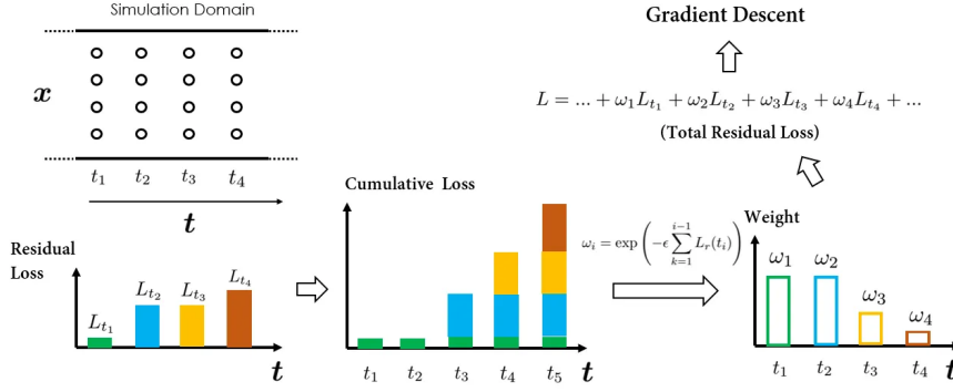
Figure 4.19: Illustration of the causal training algorithm. From [Guo24].
