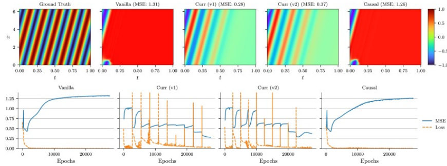
Figure 4.12: Worst case prediction for each method. The upper row shows the output of the trained network, the lower row reports the total loss and the mean squared error over the training epochs. Adapted from [MA23].
