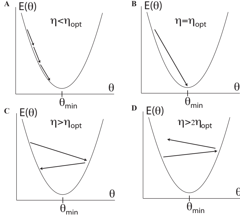
Figure 4.17: Effect of learning rate on convergence. For a one dimensional quadratic potential, one can show that there exists four different qualitative behaviours for gradient descent (GD) as a function of the learning rate \eta depending on the relationship between \eta and \eta_{\text{opt}} = [\partial_{\theta}^2 E(\theta)]^{-1} . (a) For \eta < \eta_{\text{opt}} , GD converges to the minimum. (b) For \eta = \eta_{\text{opt}} , GD converges in a single step. (c) For \eta_{\text{opt}} < \eta < 2\eta_{\text{opt}} , GD oscillates around the minima and eventually converges. (d) For \eta > 2\eta_{\text{opt}} , GD moves away from the minima. From [Meh+19], adapted from [LeC+02].
