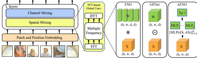
Figure 5.13: The multi-layer transformer network with FNO, GFN, and AFNO mixers. GFNet performs element-wise matrix multiplication with separate weights across channels ( k ). FNO performs full matrix multiplication that mixes all the channels. AFNO performs block-wise channel mixing using MLP along with soft-thresholding. The symbols h , w , d , and k refer to the height, width, channel size, and block count, respectively. From [Gui+21a].
