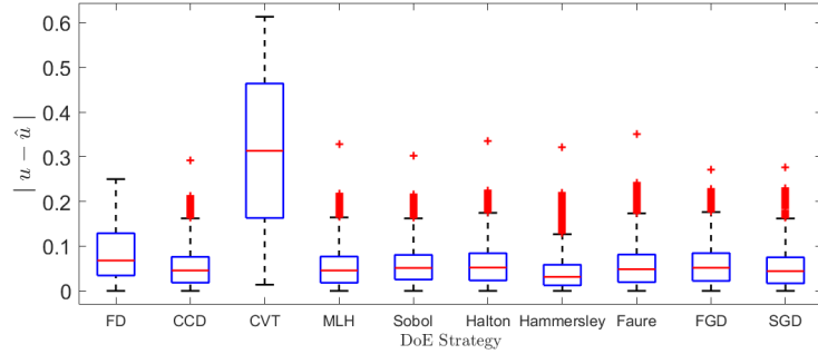
Figure 4.4: Absolute error between original and predicted responses of Heat equation considering different DoE strategies. From [DT22].
