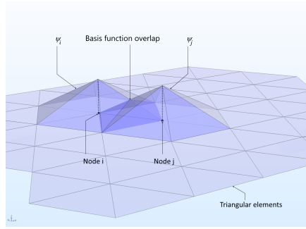
(a) Overlap between basis functions. From [Mul].
